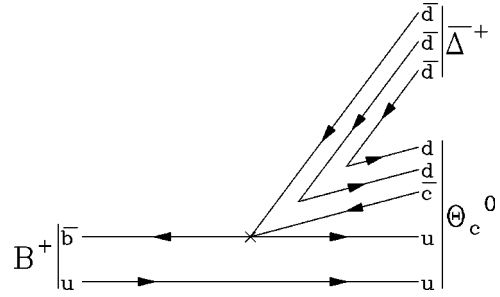
FIG. 6. Production of a charmed exotic baryon \Theta_c^0 = uud\bar{d}\bar{c} in B^+ decays.
