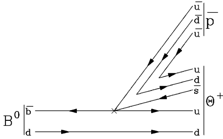
FIG. 8. Production of an exotic baryon \Theta^+ = uudd\bar{s} in B^0 decays.
