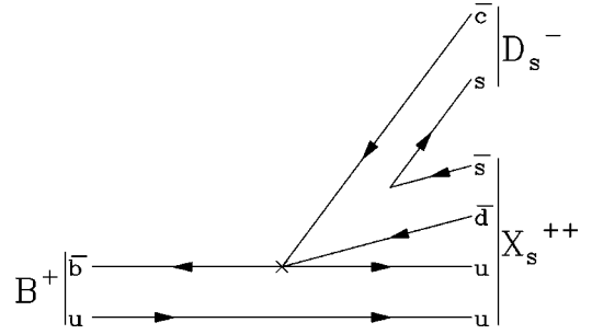
FIG. 3. Production of a strange exotic meson X^{++} = uu\bar{d}\bar{s} in B^+ decays.
